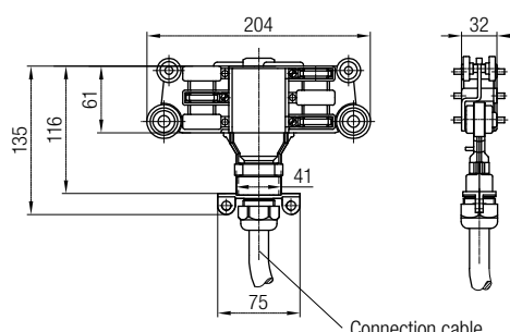
Connection cable
