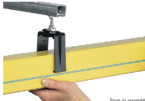
Snap-in assembly
